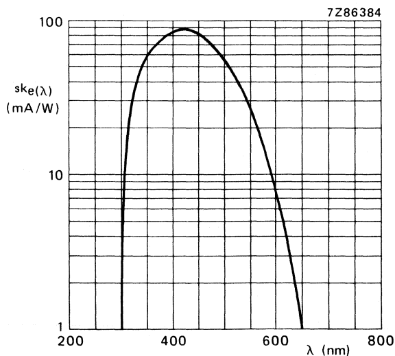
Fig. 2 Spectral sensitivity characteristic.
