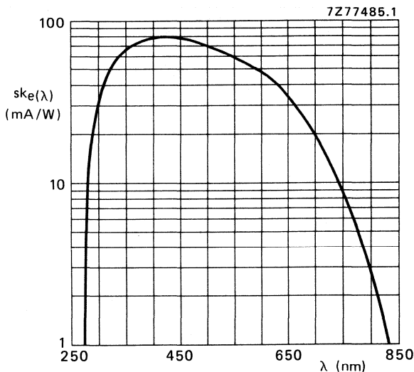
Fig. 4 Spectral sensitivity characteristic
