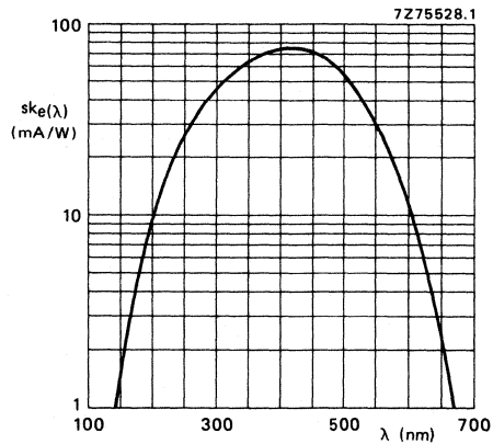
Fig. 5 Spectral sensitivity characteristic.
