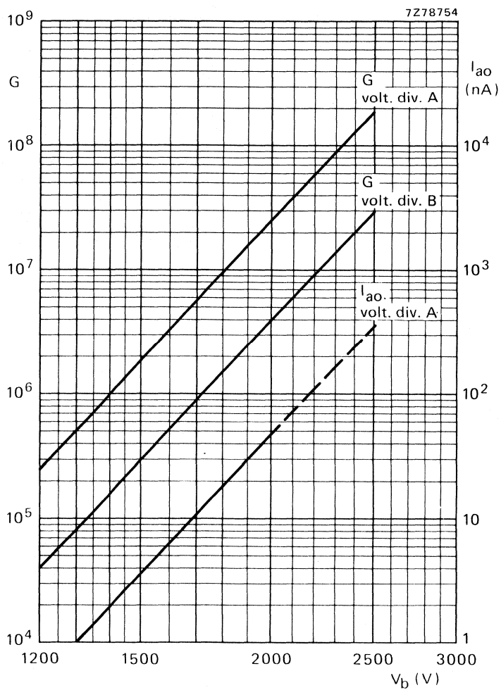
Fig. 7 Gain G , and anode dark current I_{ao} , as a function of supply voltage V_b .
