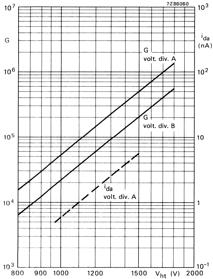
Fig. 6 Gain G and anode dark current i_{da} as a function of the supply voltage V_{ht} . i_{da} is given as a dotted line to indicate its principle behaviour only.
