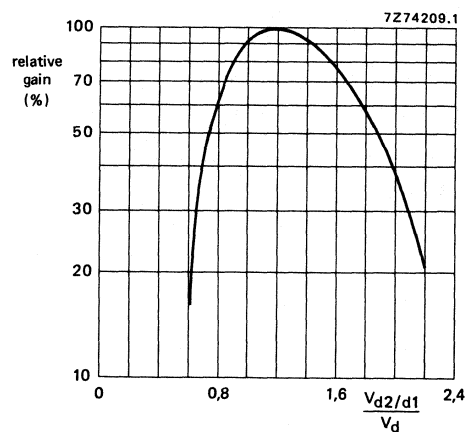
Fig. 7 Relative gain as a function of the voltage between d2 and d1, normalized to V_d . V_{d3/d1} constant.
