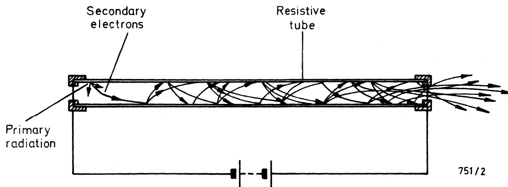
Fig.1 Electron multiplication.
