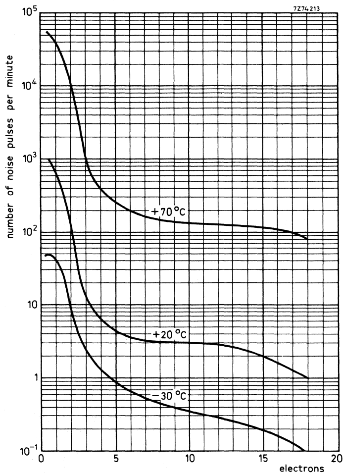
Fig. 11 Typical background spectrum from 0,1 to 18 equivalent photoelectrons, at a gain of 3 \times 10^7 with voltage divider A.
