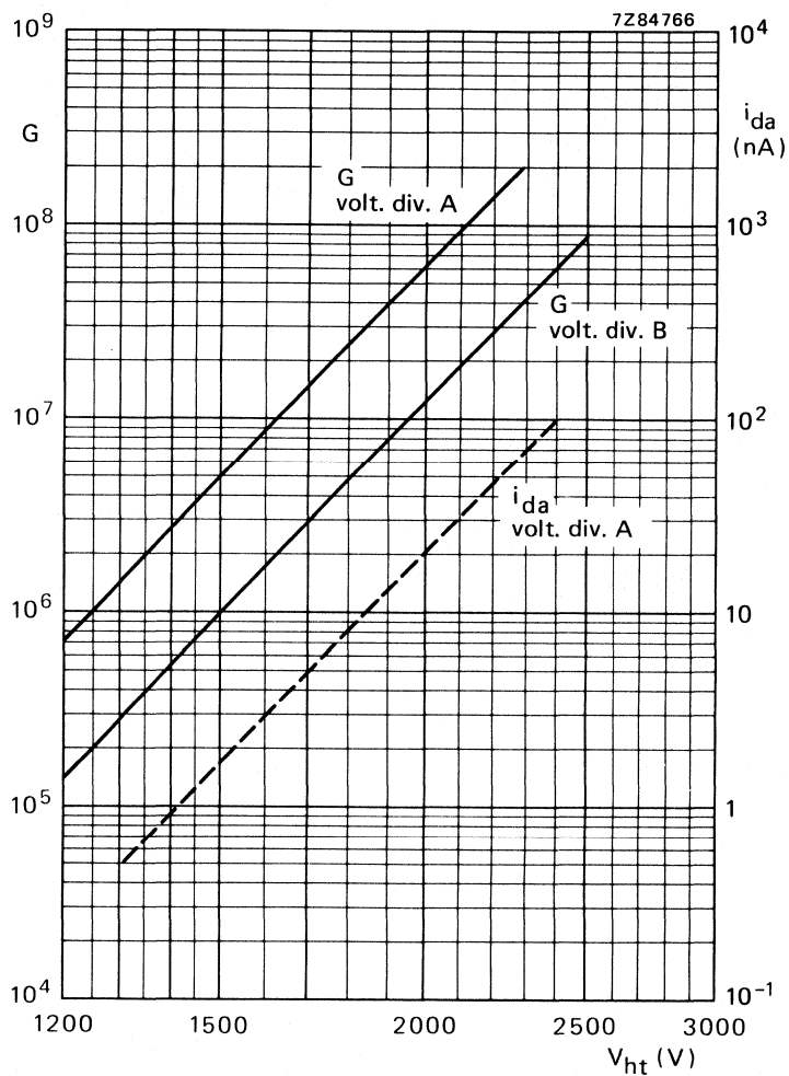
Fig. 7 Gain G and anode dark current, i_{da} , as a function of supply voltage V_{ht} ; i_{da} is given as a dotted line to indicate its principle behaviour only.
