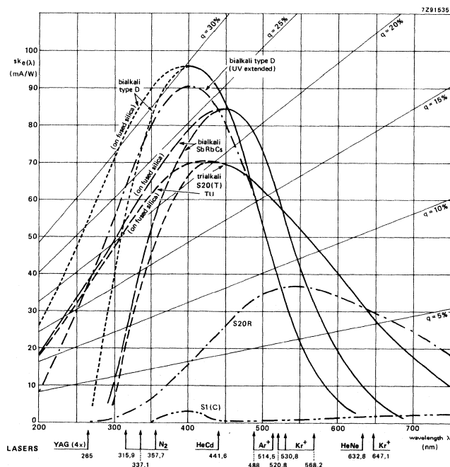
Fig.2(a) Spectral sensitivity curves of standard photocathodes, with lines of constant quantum efficiency, q , overlaid for reference. Some characteristic laser wavelengths are indicated along the wavelength axis
