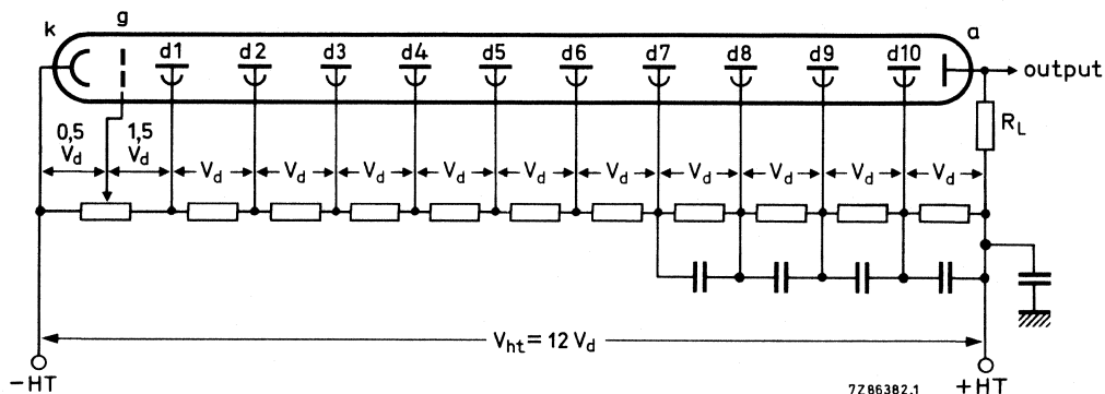
Fig. 1 Voltage divider A. Typical values of capacitors: 10 nF; k = cathode; g = accelerating electrode; dn = dynode no.; a = anode; R_L = load resistor.
