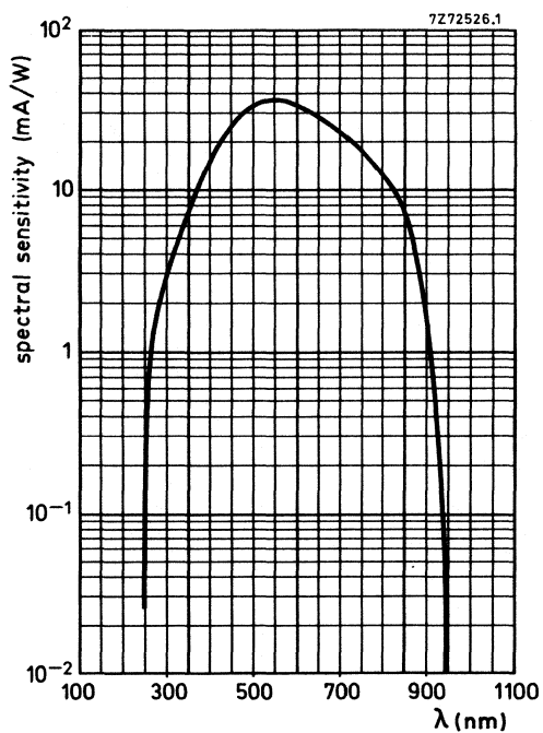
Fig. 5 Spectral sensitivity characteristic.
