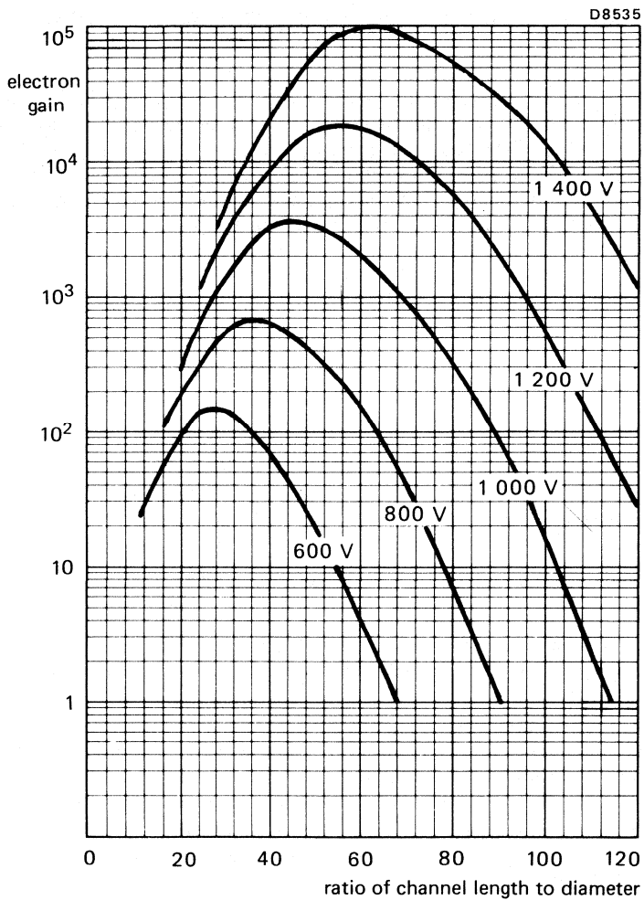
Fig.1 Typical universal gain curves
