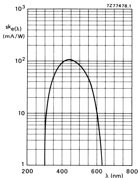
Fig. 2 Spectral sensitivity characteristic.
