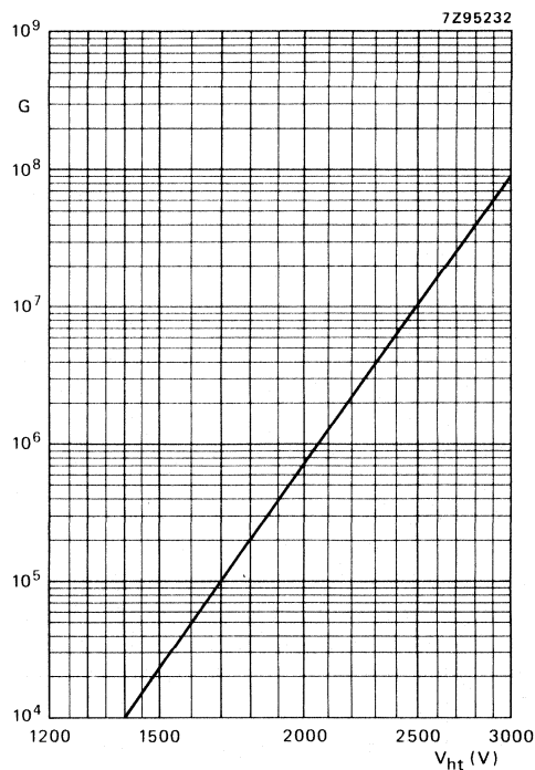
Fig. 3 Gain G as a function of supply voltage V_{ht} .
