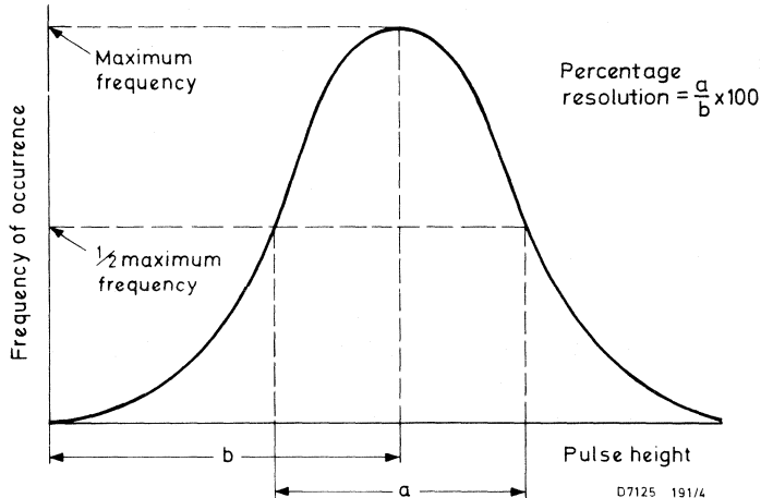
Fig.4 Definition of resolution of pulse height distribution
