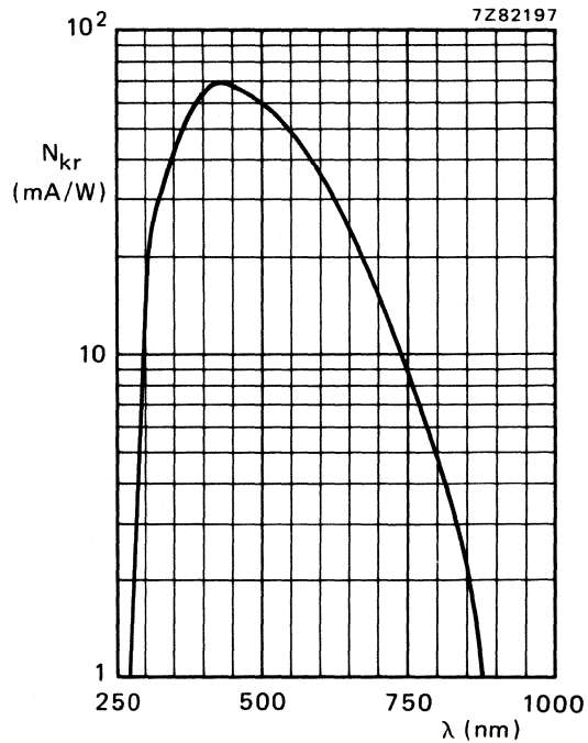
Fig. 5 Spectral sensitivity characteristic.
