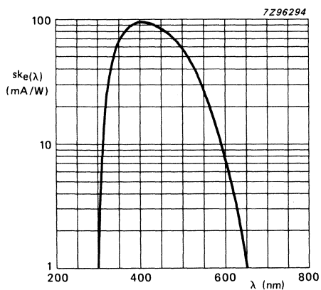
Fig. 6 Spectral sensitivity characteristic.
