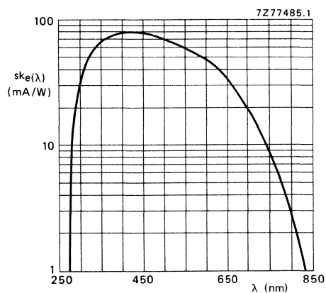
Fig. 5 Spectral sensitivity characteristic.
