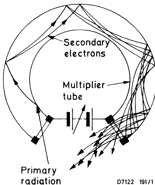
Fig.1 Electron multiplication
