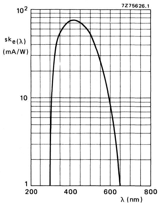
Fig. 6 Spectral sensitivity characteristic.
