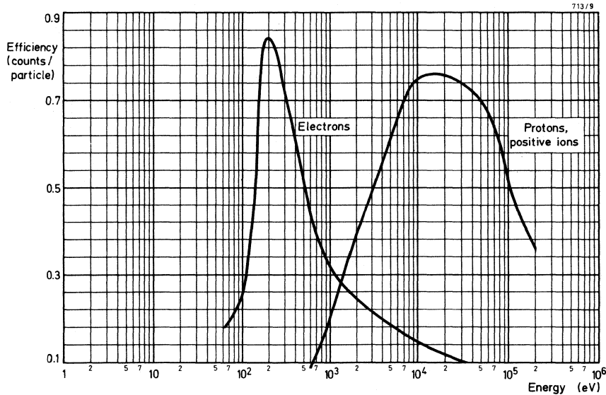
Fig.7 Typical detection efficiencies for electrons, protons and positive ions
