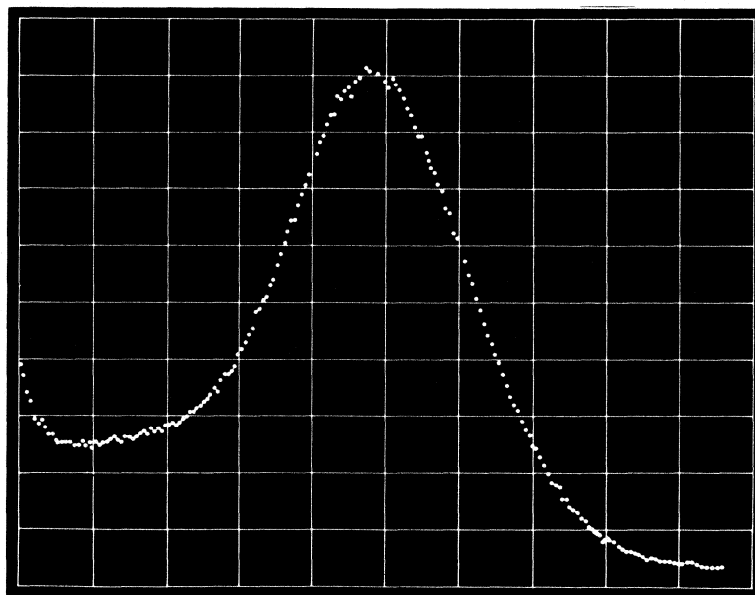
Fig. 7 Single electron spectrum obtained with an XP2262 tube.
