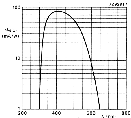
Fig. 4 Spectral sensitivity characteristic.
