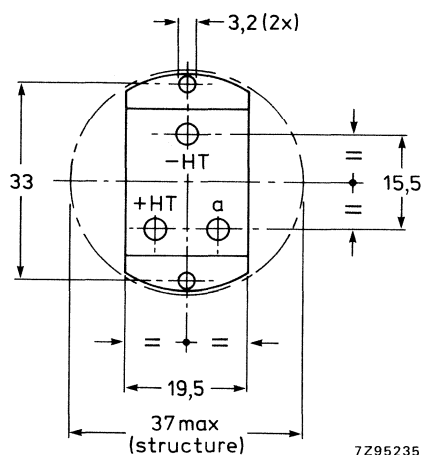
Bottom view of metal clamp.
