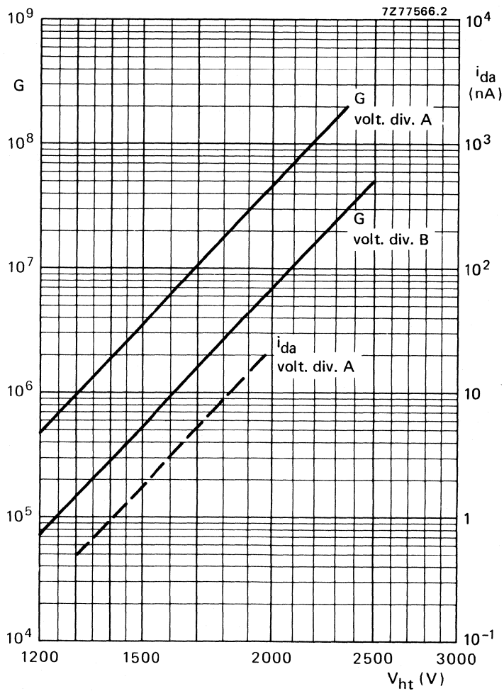
Fig. 8 Gain G and anode dark current, i_{da} , as a function of supply voltage V_{ht} .
