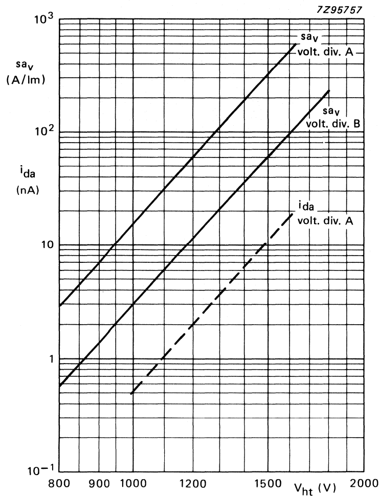
Fig. 6 Anode luminous sensitivity s_{av} and anode dark current i_{da} as a function of the supply voltage V_{ht} . i_{da} is given as a dotted line to indicate its principle behaviour only.
