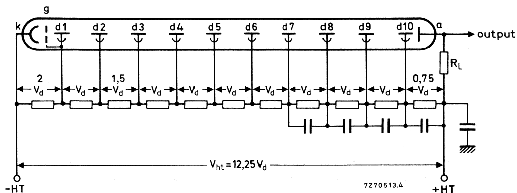
Fig. 2 Voltage divider A. Typical values of capacitors: 10 nF; k = cathode; g = accelerating electrode; dn = dynode no.; a = anode; R_L = load resistor.
