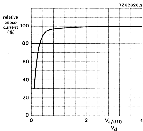
Fig. 6 Relative anode current as a function of the voltage between anode and final dynode. V_d = 90 V.
