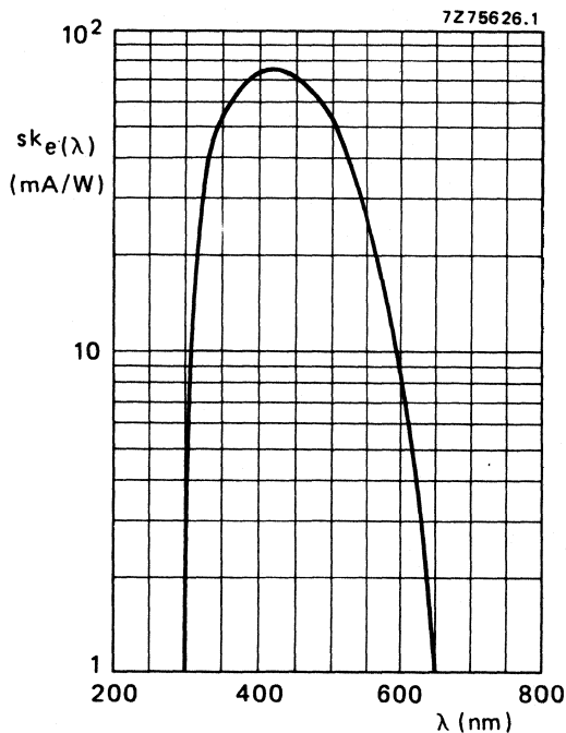
Fig. 4 Spectral sensitivity characteristic.
