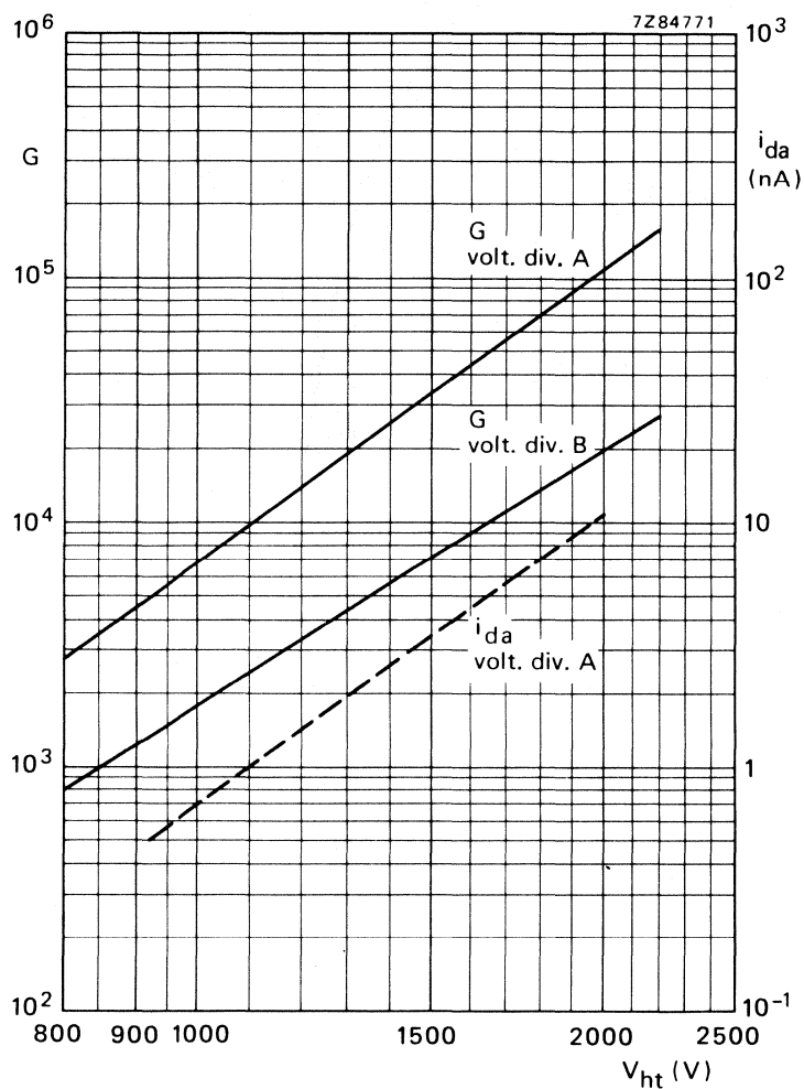
Fig. 6 Gain G and anode dark current, i_{da} , as a function of supply voltage V_{ht} .
