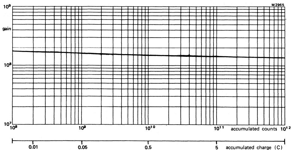
Fig.9 Typical gain as a function of accumulated counts and accumulated charge for the X900 series of single channel electron multipliers. Operating voltage = 2.8 kV, ambient pressure = 0.013 \text{ mN.m}^{-2} ( 1.3 \times 10^{-7} mbar), counting rate = 10^4 count/s, source: electrons.
